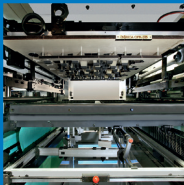
Stripping Frames with quick lock systems and position regulators
