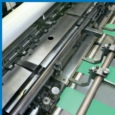
Double function Side guides. Inductive motorized Front lays
