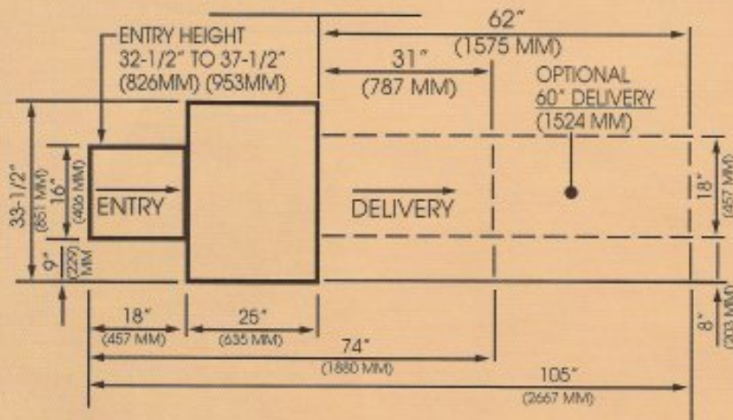
Horizontal Floor Plan
