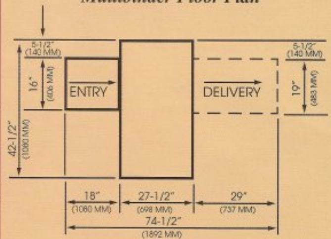
Multibinder Floor Plan
