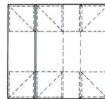
6-corner glued collapsible box
