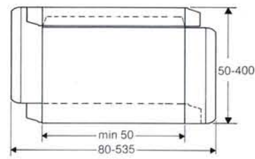
Straight-line folding carton
