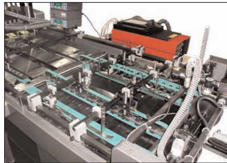
Converting Area
